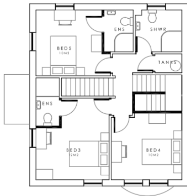
PROPOSED FIRST FLOOR 1:100
